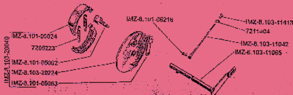
Fig35.Frein side car
