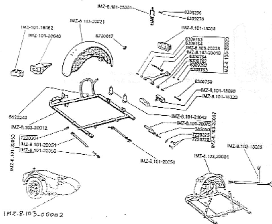
Fig33.Side car
