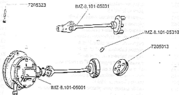
Fig12.Pont/Arbre de transmission
